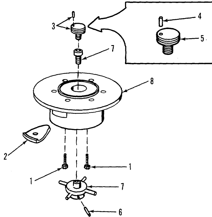
Figure 28. Rifle mount adapter assembly and collar and pin assembly.
